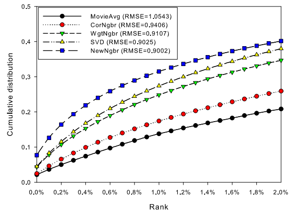
Figure 3: Comparing the performance of five methods on a top-K recommendation task, where a few products need to be suggested to a user. Values on the x -axis stand for the percentile ranking of a 5-star rated movie; lower values represent more successful recommendations. We experiment with 384,573 cases and show the cumulative distribution of the results. The plot concentrates on the more relevant region, pertaining to low x -axis values. The new neighborhood method has the highest probability of placing a 5-star rated movie within the top-K recommendations. On the other hand, the non-personalized MovieAvg method and the popular correlation-based neighborhood method (CorNgbr) achieve the lowest probabilities.
